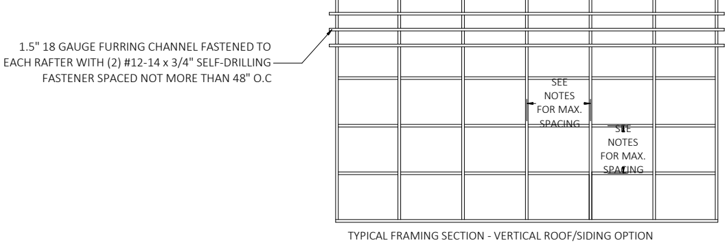
TYPICAL FRAMING SECTION - VERTICAL ROOF/SIDING OPTION
