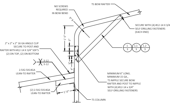
SIDE EXTENSION RAFTER/COLUMN DETAIL FOR EXTENSION RAFTER SPANS 12'-0" < W <= 16'-0", IF THE KNEE BRACE ON THE OTHER END OF THE RAFTER IS PER DETAIL 1.2/3 FOR EXTENSION RAFTER SPANS 13'-0" < W <= 18'-0", IF THE KNEE BRACE ON THE OTHER END OF THE RAFTER IS PER DETAIL 1.1/3 FOR EXTENSION RAFTER SPANS 15'-0" < W <= 19'-0", IF THE KNEE BRACE ON THE OTHER END OF THE RAFTER IS PER DETAIL 1/3. SCALE: NTS
