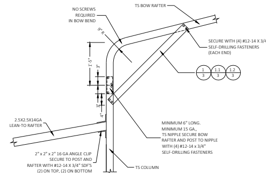
SIDE EXTENSION RAFTER/COLUMN DETAIL FOR EXTENSION RAFTER SPANS W' < 12'-0" , IF THE KNEE BRACE ON THE OTHER END OF THE RAFTER IS PER DETAIL 1.2/3 FOR EXTENSION RAFTER SPANS W' < 13'-0" , IF THE KNEE BRACE ON THE OTHER END OF THE RAFTER IS PER DETAIL 1.1/3 FOR EXTENSION RAFTER SPANS W' < 15'-0" , IF THE KNEE BRACE ON THE OTHER END OF THE RAFTER IS PER DETAIL 1/3. SCALE: NTS
