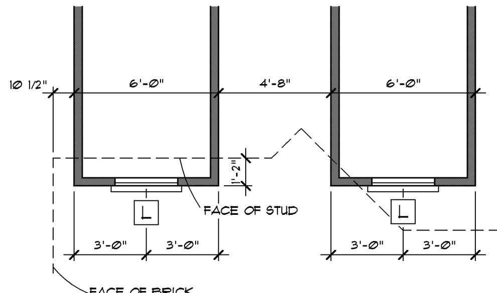
DORMER PLAN
