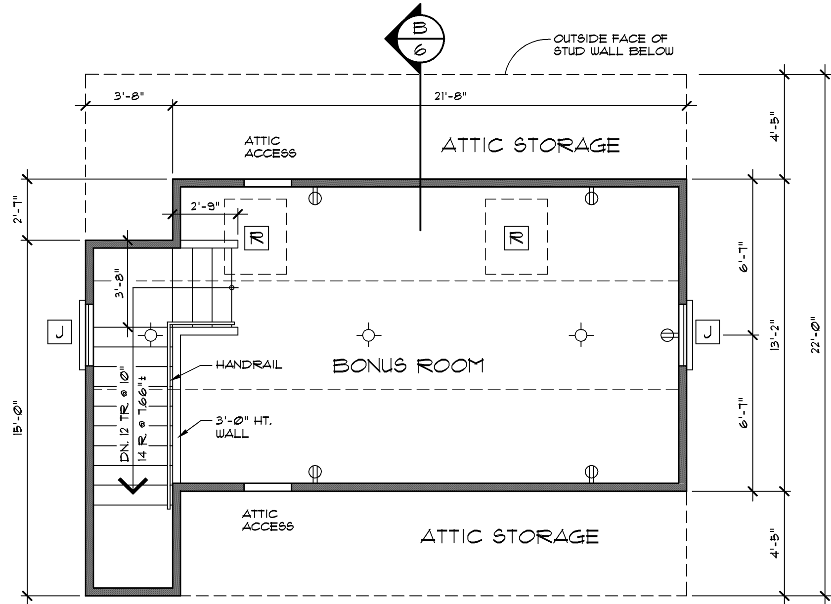
BONUS ROOM FLOOR PLAN
