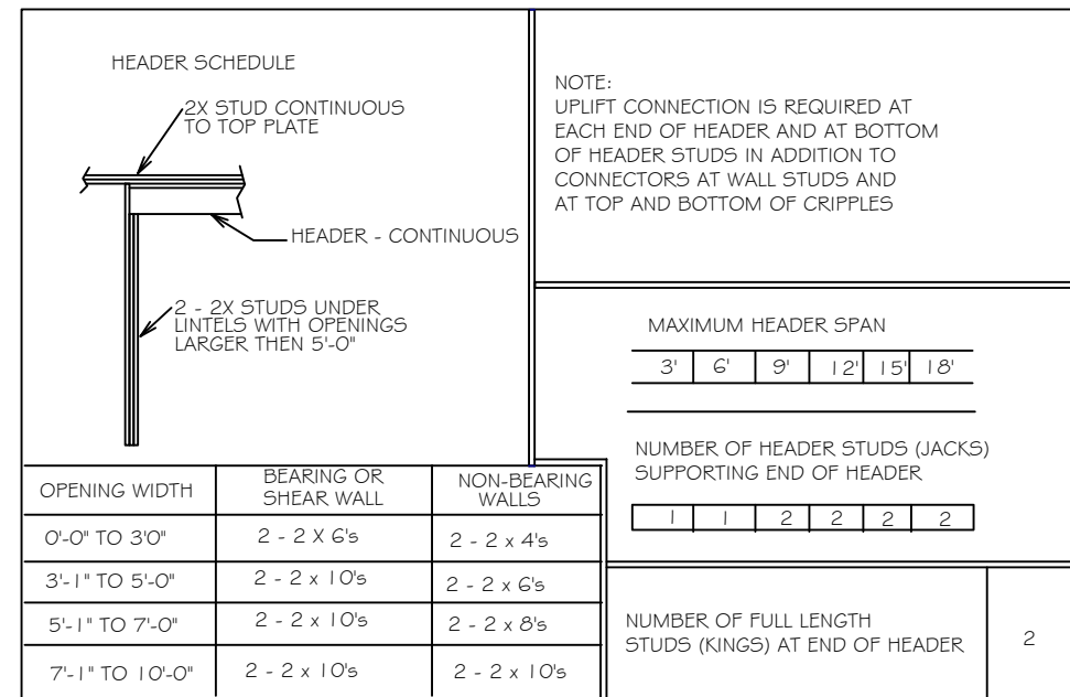
TYPICAL HEADER STRAPPING NOT TO SCALE
