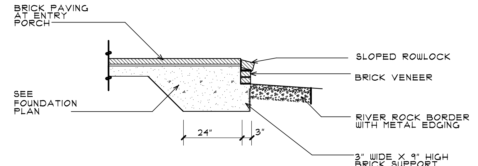
ALTERNATE ONE FRONT PORCH WITH BRICK VENEER AND PAVING SCALE 1/2" = 1'-0"
