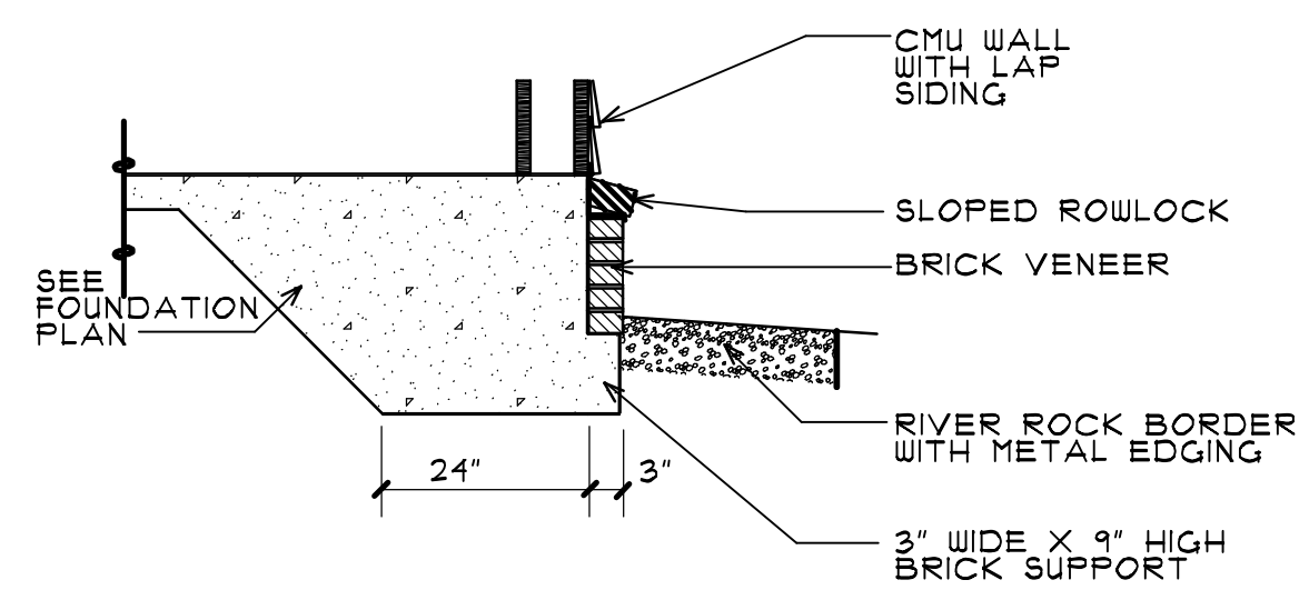
ALTERNATE ONE FOUNDATION WITH BRICK VENEER SCALE 1/2" = 1'-0"
