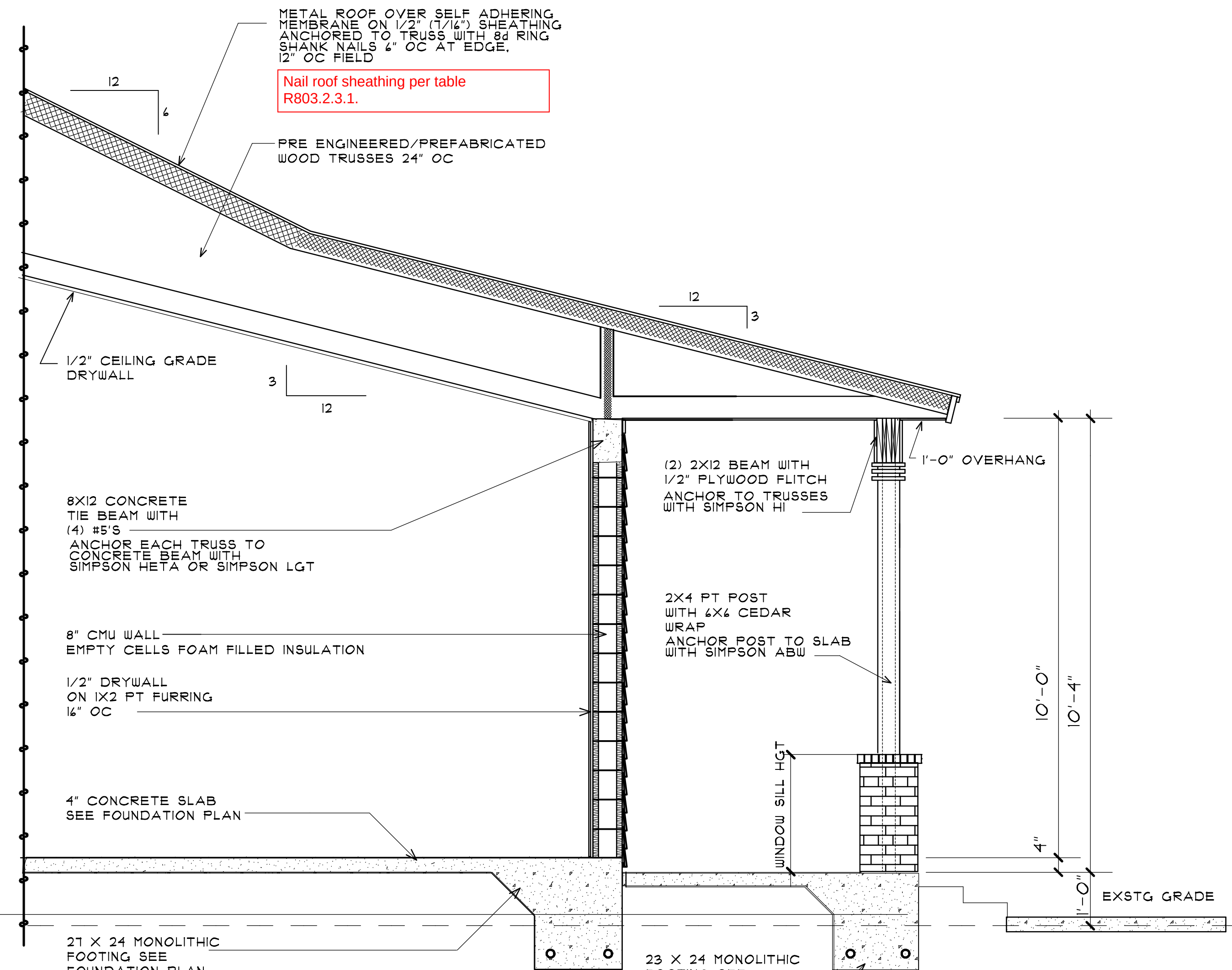
B SECTION THRU EAST PORCH SCALE 1/2" = 1'-0"
