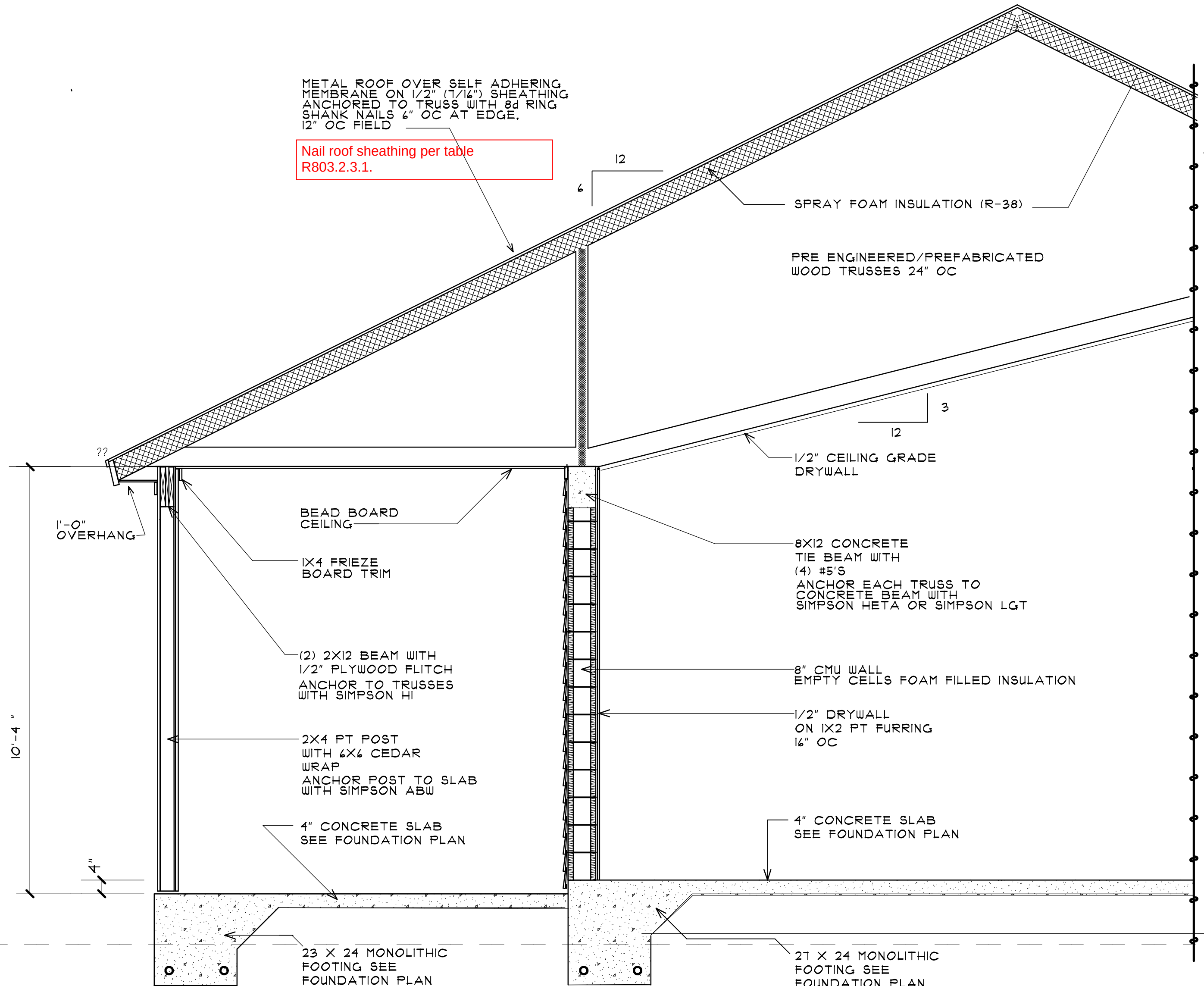
A SECTION THRU WEST SCREENED PORCH SCALE 1/2" = 1'-0"
