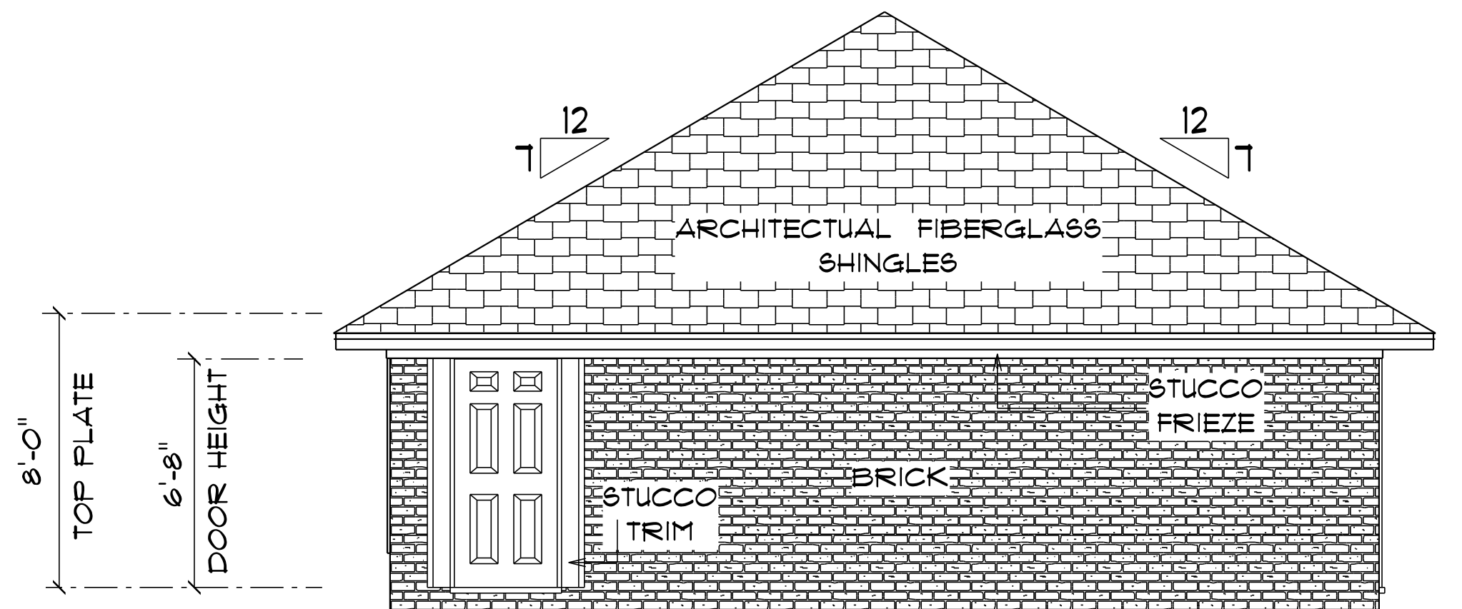
* PARTIAL * * REAR ELEVATION *
