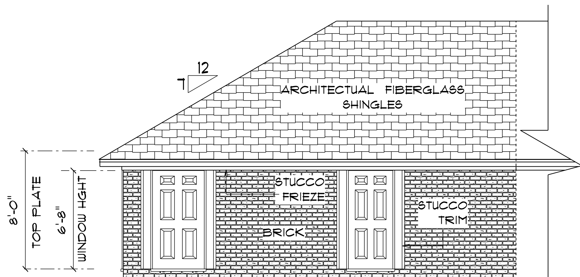
* PARTIAL * * LEFT SIDE ELEVATION *
